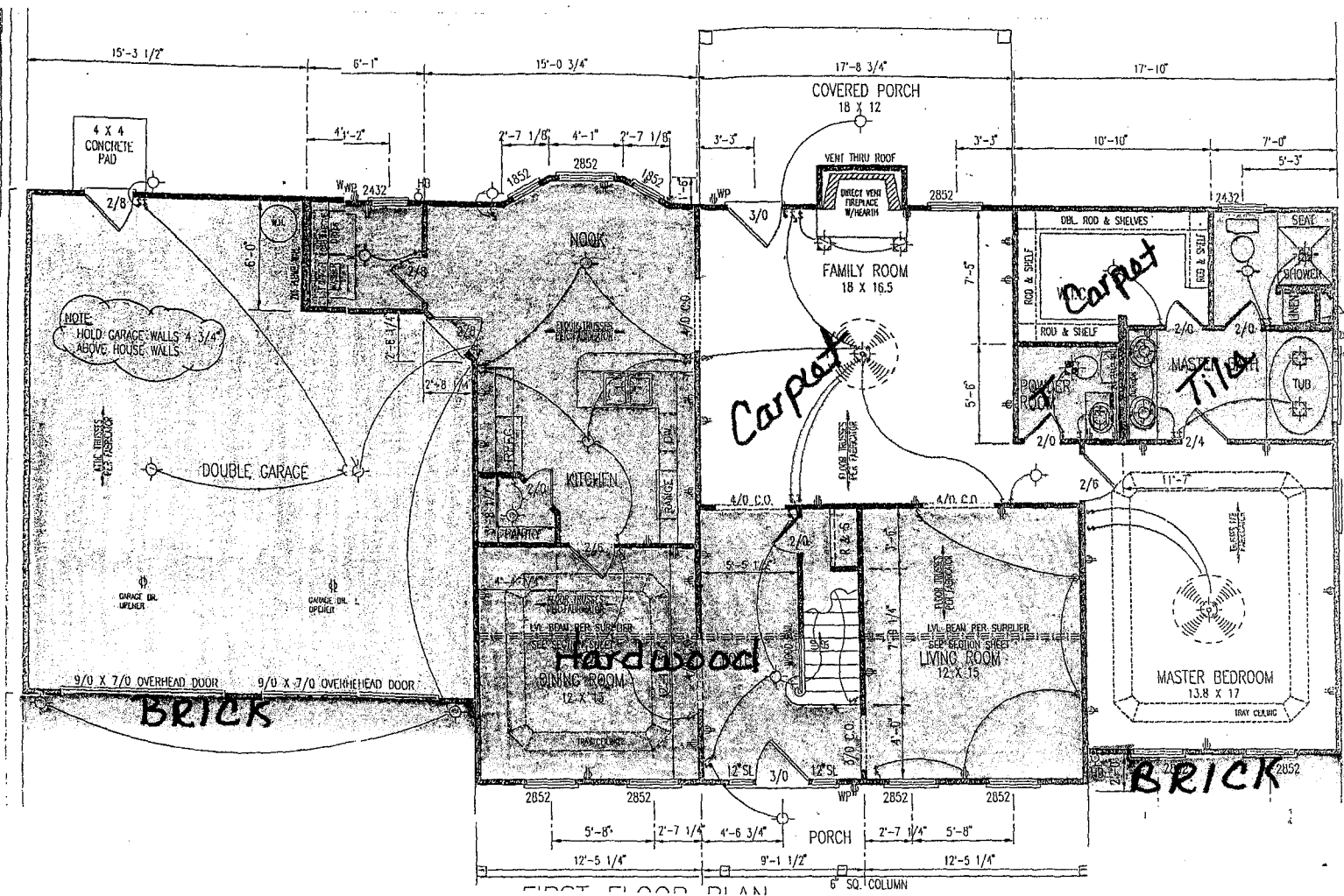
FIRST FLOOR PLAN 6" SQ. COLUMN
