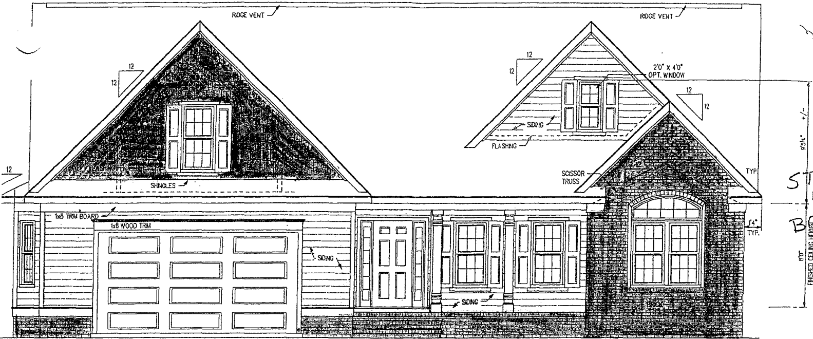
FRONT ELEVATION
